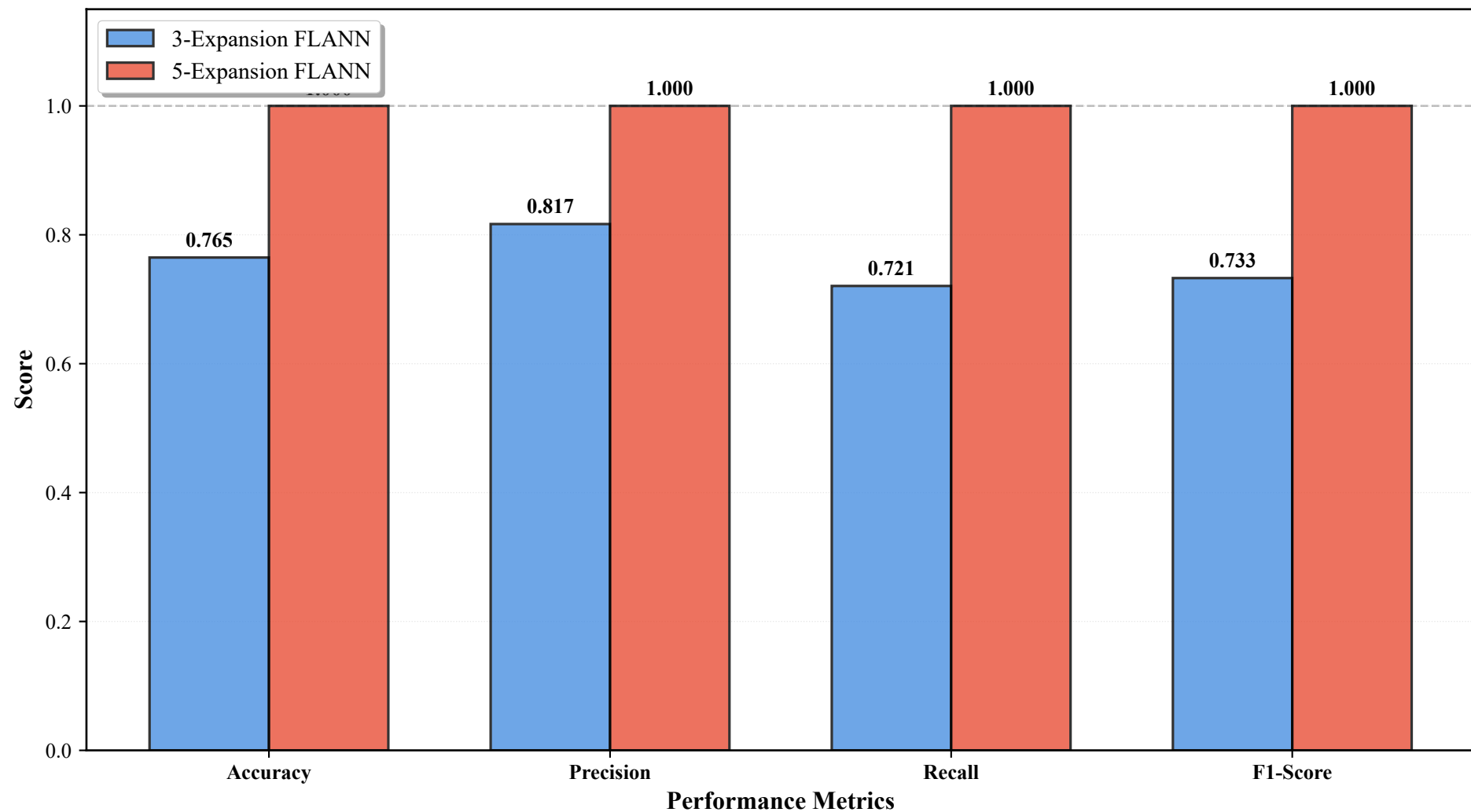
Performance Metrics Comparison: 3-Expansion vs 5-Expansion FLANN
